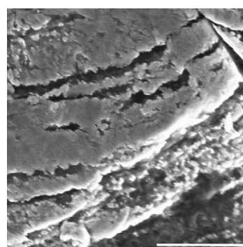
Figure 5. SEM image of the Pd foil in spot-heated experiment showing a section adjacent to the heated area where significant Pd re-deposition has taken place. Scale bar 5 \mu\text{m} .
