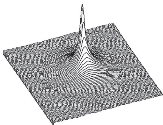
Figure 3. Image of the Pd foil (250 \mu\text{m} ) recorded with an IR camera (FLIR ThermoCAM SC1000). The tip of a soldering iron heated to 400°C was held approximately at the center of the foil underneath the reactor. To record the heat distribution, the Pd foil was coated with soot to decrease reflectance, while mounted on a heat sink held at 37°C.
