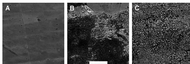
Figure 4. SEM images of the surface of the Pd foil after treatment with spot heater. A) Pd surface outside the heated zone but still exposed to the reactants; B) the transition between heated and not-heated areas of the Pd surface and resultant pitting of the surface; C) Pd surface inside the heated zone where reaction takes place. Scale bar 20 \mu\text{m} .
