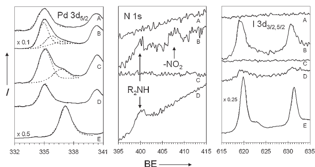
Figure 2. X-ray photoelectron spectra: A) Pd foil washed with DMF; B) Pd foil after the Suzuki–Miyaura coupling reaction; C) sample B after prolonged washing with DMF; D) Pd foil exposed to a solution of p -iodonitrobenzene in DMF, E) PdI 2 .
